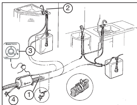
Plan for warm water supply
