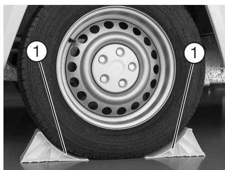
Place the wheel chocks in front of and behind the wheel
