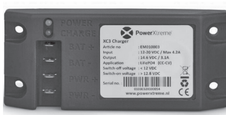
Charge booster
