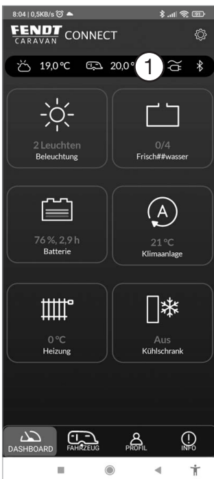
User interface
